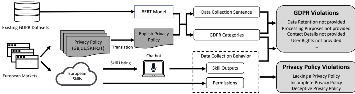
Figure 1: Methodology Overview
